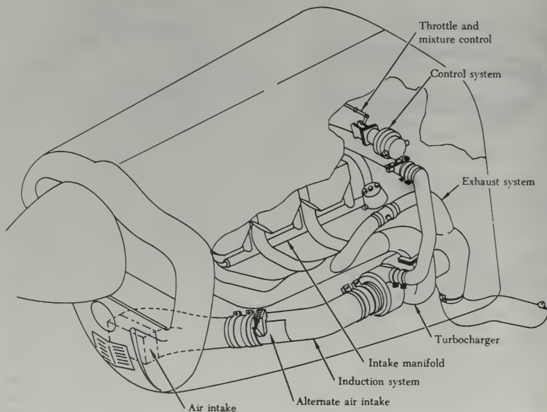
FIGURE 2-13. Turbocharger induction and exhaust systems.
